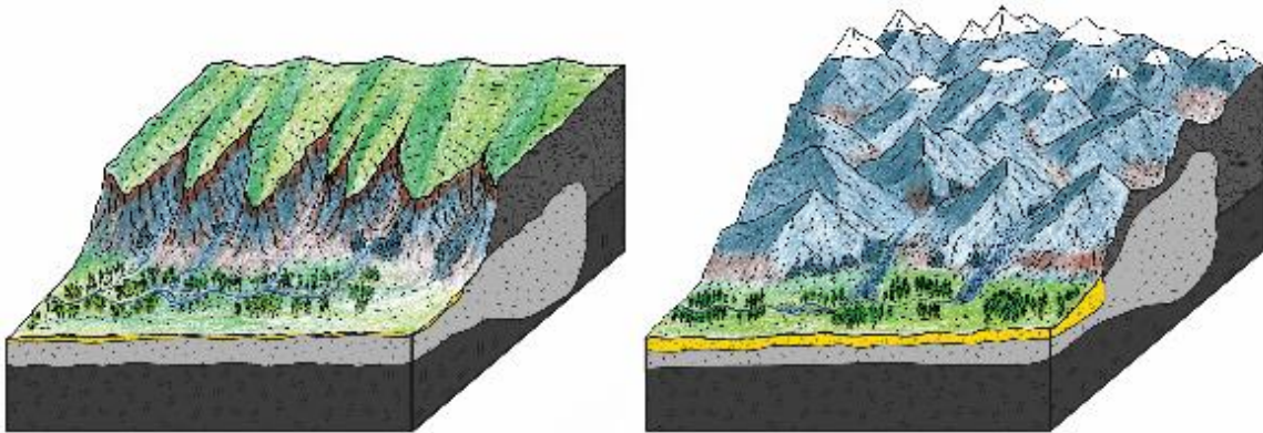
Headwaters of Alpine streams approximately 30 million years ago (left) with an Alpine plateau and a meadow countryside. The handcraft on the right side illustrates the landscape of the Alps at 25 million years before present with steep valleys where torrents originated. © Philippos Garefalakis, University of Bern.
